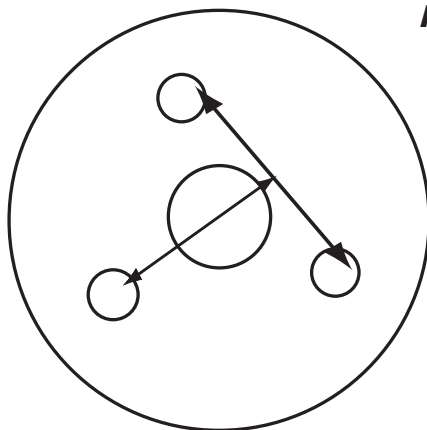
3-LUG – Middle of one hole to outside line across other two holes (example 3/100)
