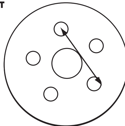
5-LUG – Back of one hole to the center of the second hole (example 5/130) (NOTE: This is the easiest way we know to estimate the 5-lug bolt circle.)
