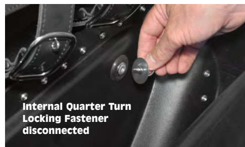
Internal Quarter Turn Locking Fastener
